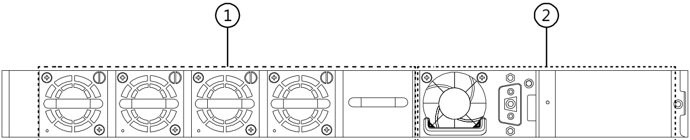
Figure 4-4 Back Panel of SNQ-60x0-320F Series Switch with DC Power Supply Module
