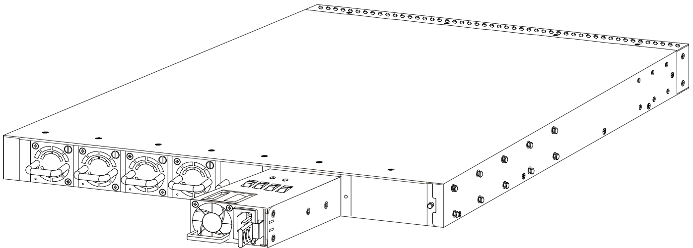
Figure 5-7 Installing an AC Power Supply Module (Before)
