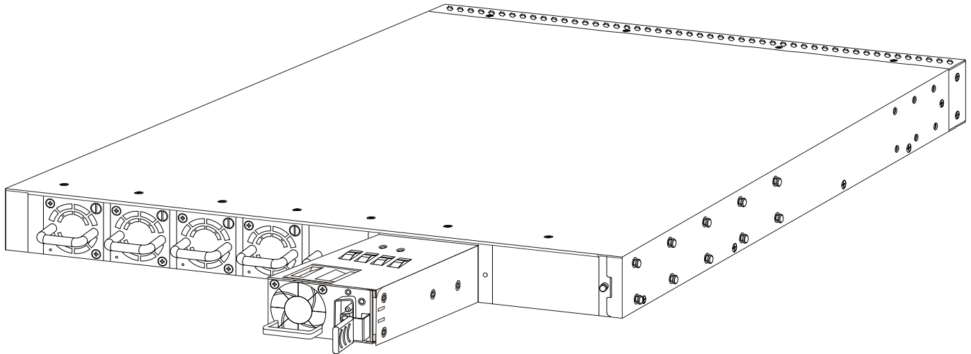
Figure 5-9 Installing a DC Power Supply Module (Before)
