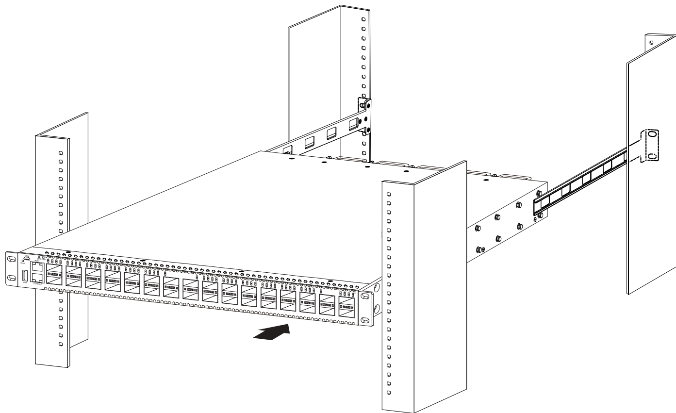
Figure 5-4 Slide switch into position
