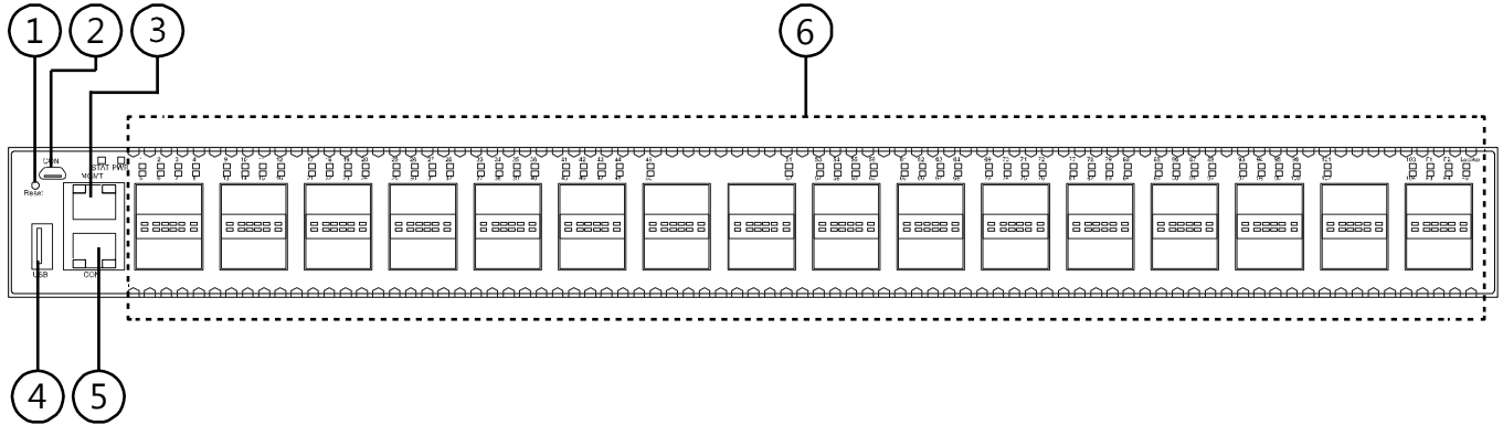
Figure 4-1 Front Panel of SNQ-60x0-320F Series Switch (Ports)
