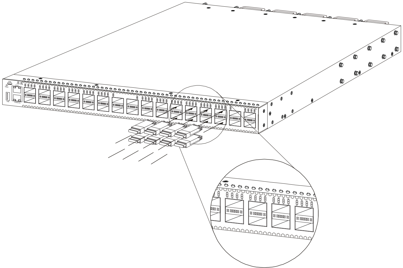
Figure 5-6 Installing Transceivers into the Transceiver Ports
