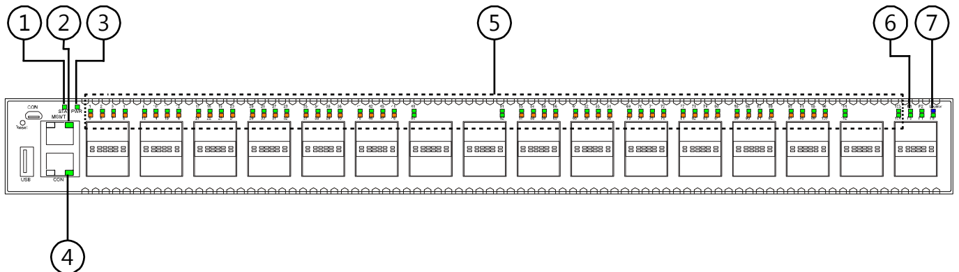
Figure 4-2 Front Panel of SNQ-60x0-320F Series Switch (LED Indicators)
