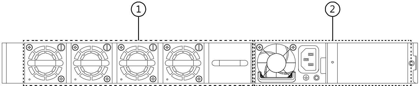
Figure 4-3 Back Panel of SNQ-60x0-320F Series Switch with AC Power Supply Module
