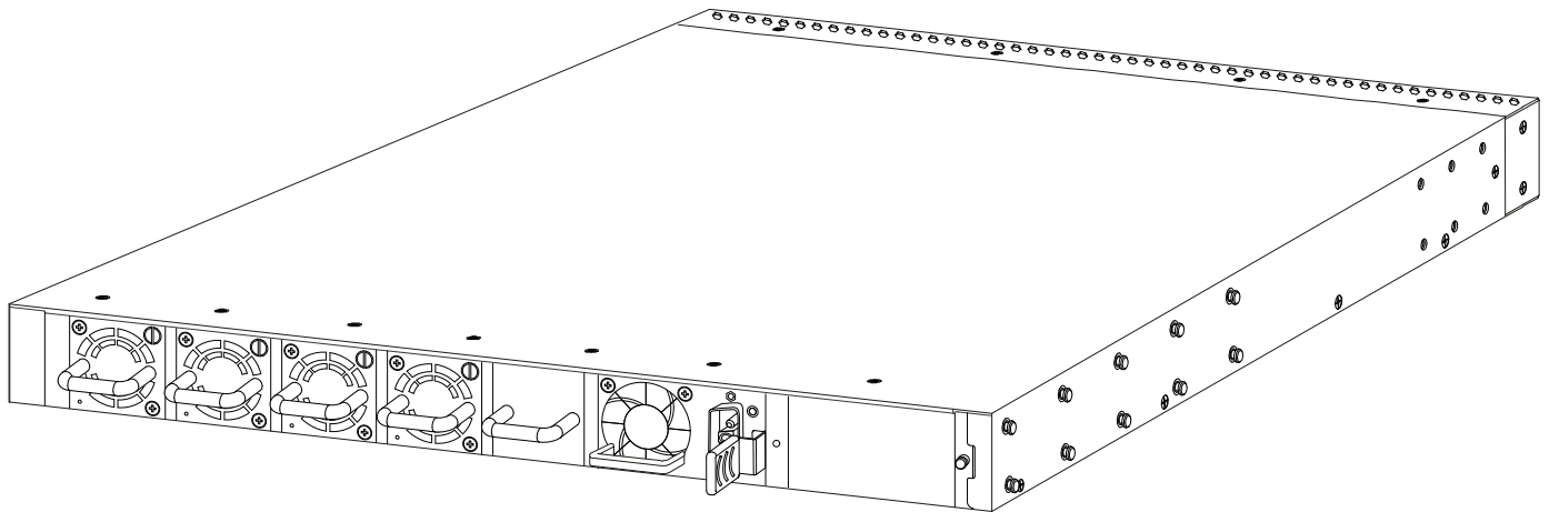
Figure 5-10 Installing a DC Power Supply Module (After)
